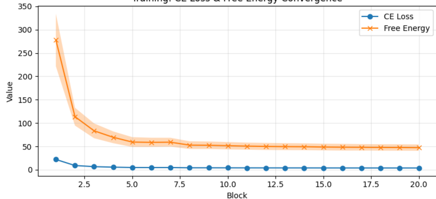
Training: CE Loss &amp; Free Energy Convergence
