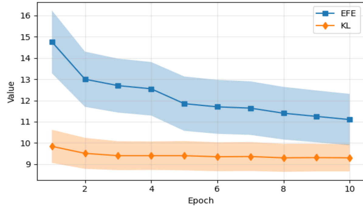
Training: Free Energy Decomposition
