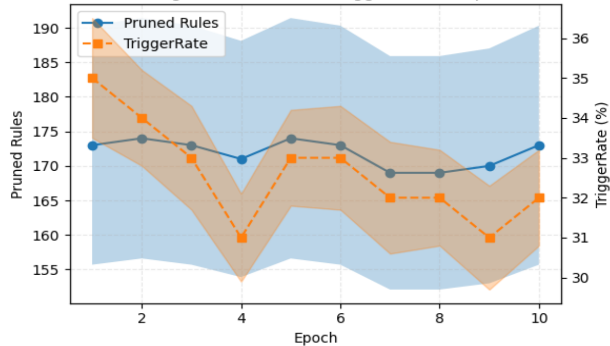
Training: Pruned Rules &amp; TriggerRate vs Epoch
